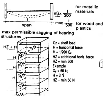
⑤ Assumed loads for storage equipment
